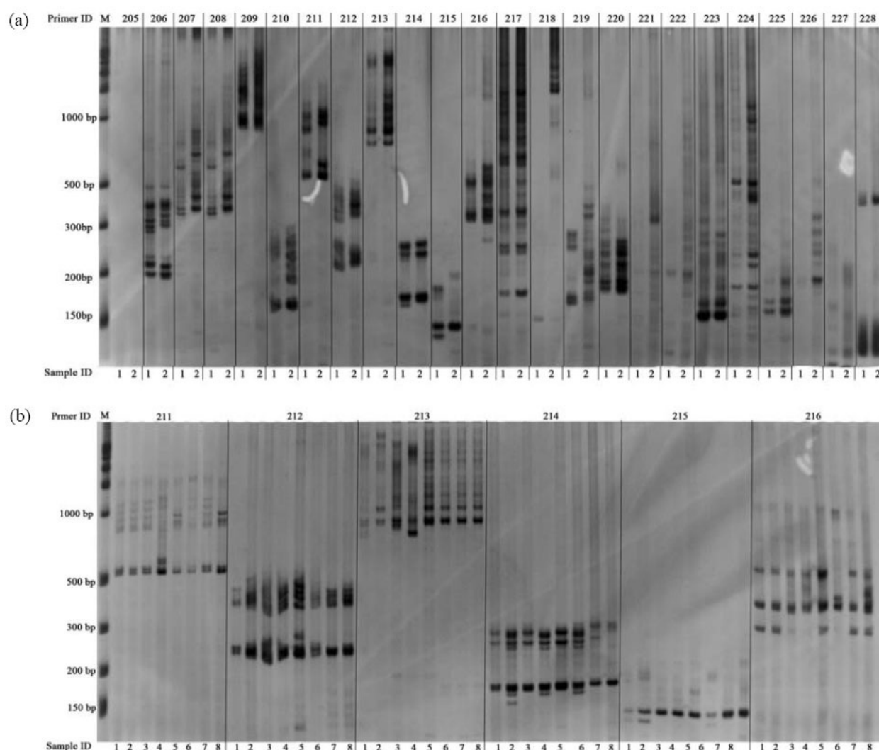
Figure 3 Examples of PCR products amplified by SSR primer pairs. (a) PCR products amplified by 24 primer pairs (GDAAS 205-228 listed on the top of the gel image) in E Shu 3 Hao (gel lanes 1 labeled in each SSR primer pair panel below the bottom of the gel image) and Guang 2K-30 (lanes 2). (b) PCR products in eight sweetpotato cultivars amplified by six effective SSR primer pairs selected from figure 3a. Within each primer pair image panel, the order of DNA samples from left to right is NANCY HALL (lanes 1), Sheng Li Bai Hao (lanes 2), AB940078-1 (lanes 3), Nortnigo (lanes 4), Tai Nong 57 (lanes 5), Hua Bei 553 (lanes 6), Yu Bei Bai (lanes 7), and Bao Ting Zhong (lanes 8). Standard size markers are given on left side.
