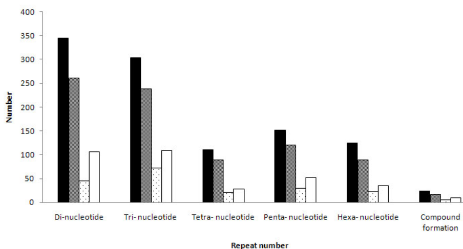
Figure 2 Number of designed primer pairs and polymorphic primer pairs. Number of primer pairs designed (black columns), primer pairs amplified (gray columns), polymorphic loci in two parents of our mapping population (dotted white columns) and polymorphic loci in the eight diverse sweetpotato cultivars (white columns).
