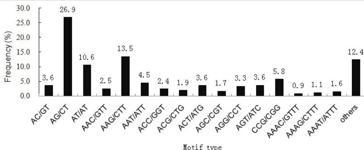
Figure 1 Frequency distribution of EST-derived SSRs of sweetpotato based on motif sequence types. X-axis is motif sequence types, and Y-axis represents the frequency of SSRs of a given motif sequence type.
